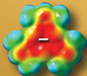
\{[3,5-(\text{CH}_3)_2\text{Pz}]\text{Au}\}_3
