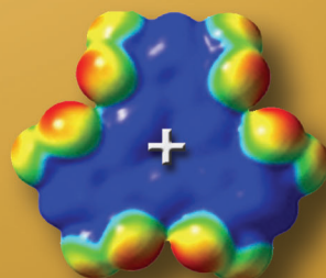
\{[3,5-(\text{CF}_3)_2\text{Pz}]\text{Au}\}_3
